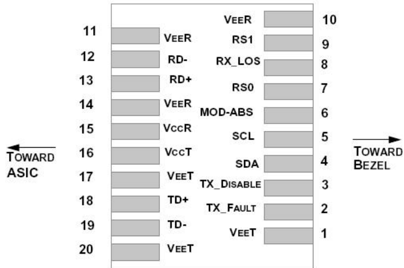
Figure 3 Pin View for SFP28
