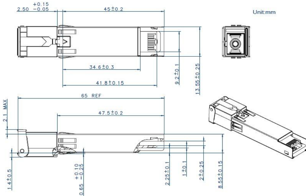
Figure 3 Package Outline
