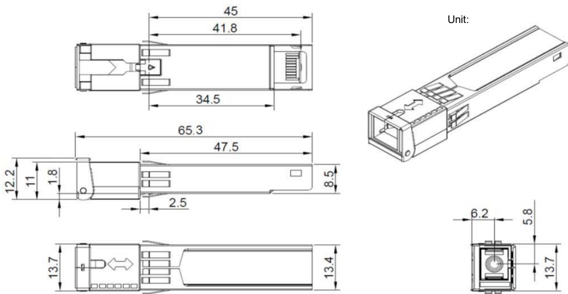
Figure 3 Package Outline
