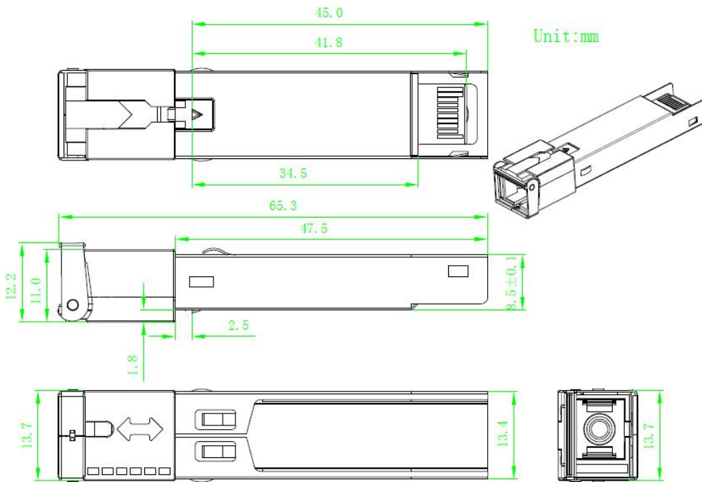
Figure 8 Package Outline
