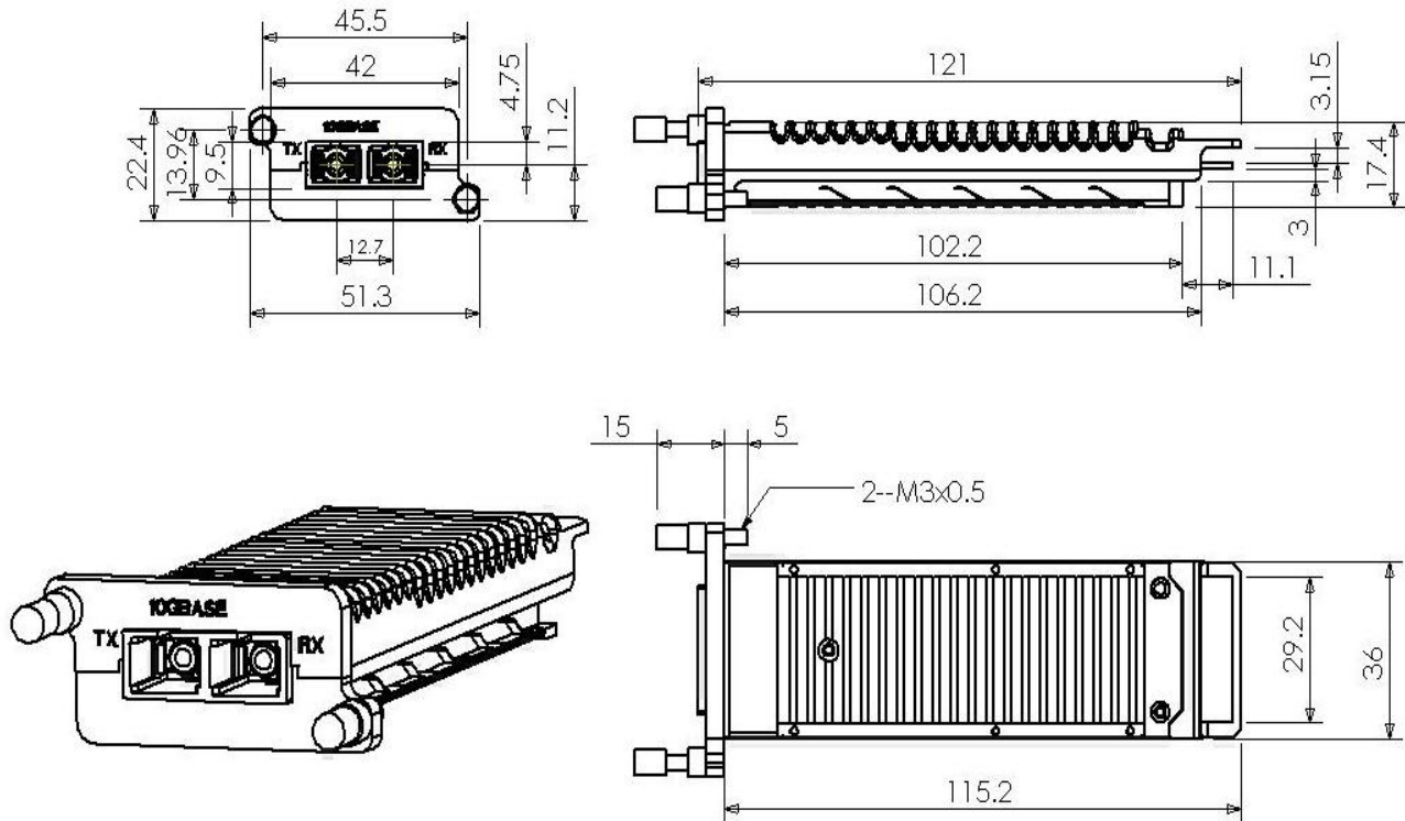
Figure 1 Mechanical dimensions
