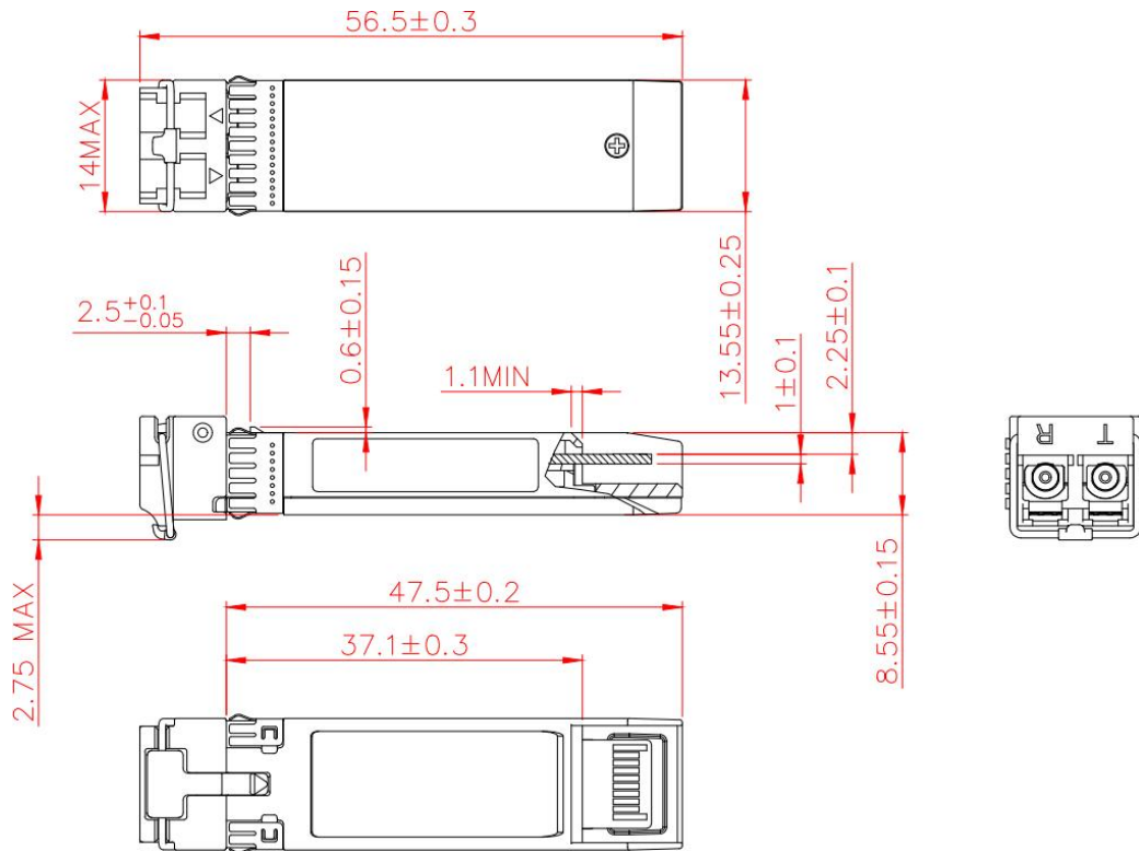
Figure 3. Module Mechanical Dimensions
