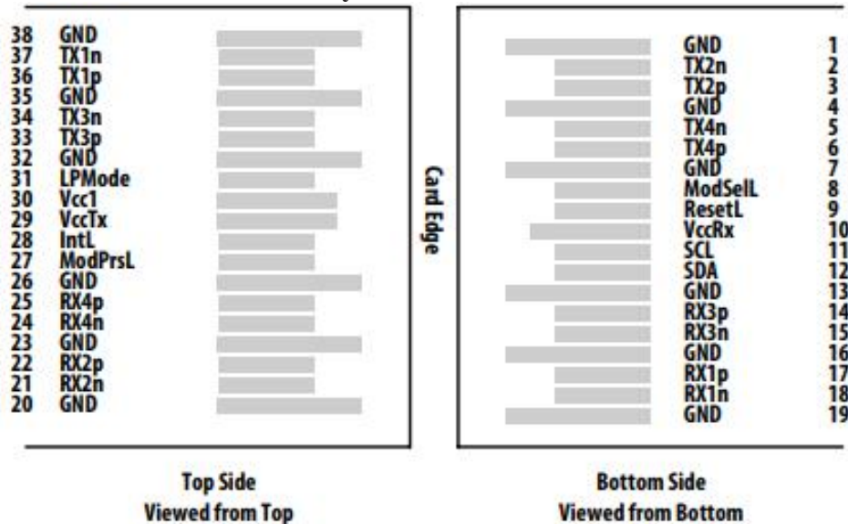
Figure 7. QSFP+ Transceiver Pad Layout
