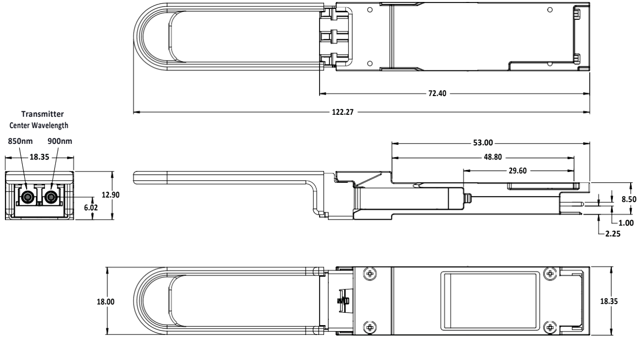
Figure 13. Mechanical Package Outline
