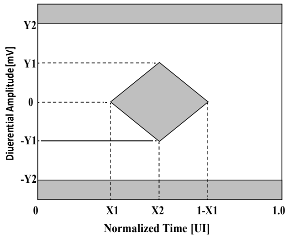
Figure 4. Rx Electrical Eye Mask Coordinates (TP4) at Hit ratio 5 \times 10^{-5} hits per sample
