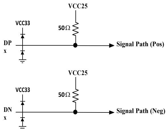
Figure 10. Transmitter Data Input Equivalent Circuit
