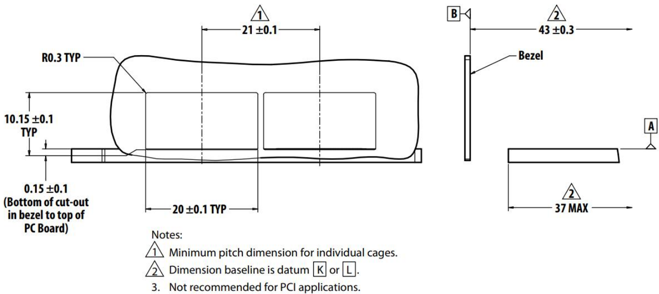
Figure 16. Host Board Bezel Design
