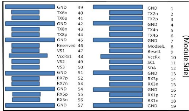
Bottom side viewed from bottom Additional QSFP-DD Pads Legacy QSFP28 Pads MSA Compliant Connector
